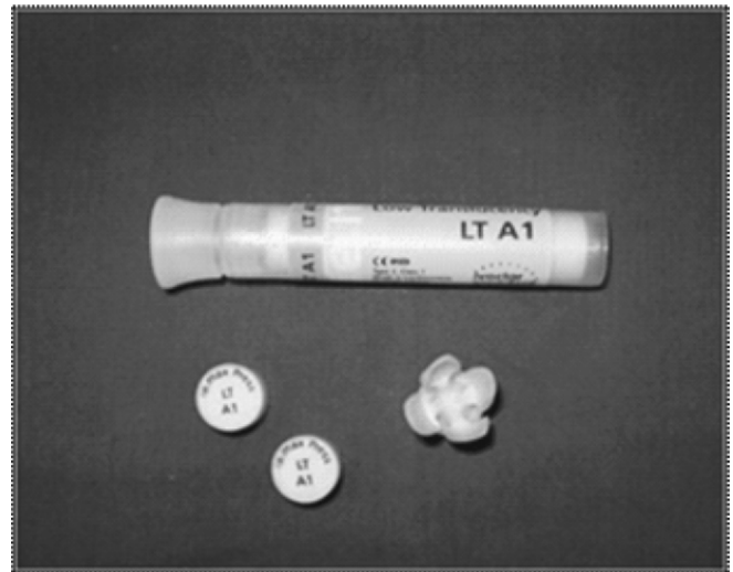
Figure 6: IPS e.max Press ingots and divested and sandblasted laminates.
