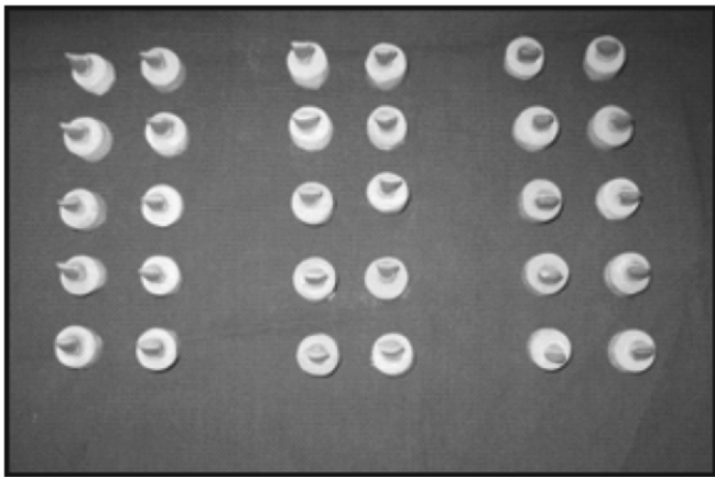
Figure 4: Prepared dies.
