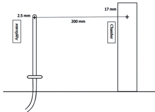
Figure 2: Experimental arrangement of the HDR applicator and chamber in air equivalent phantom.
