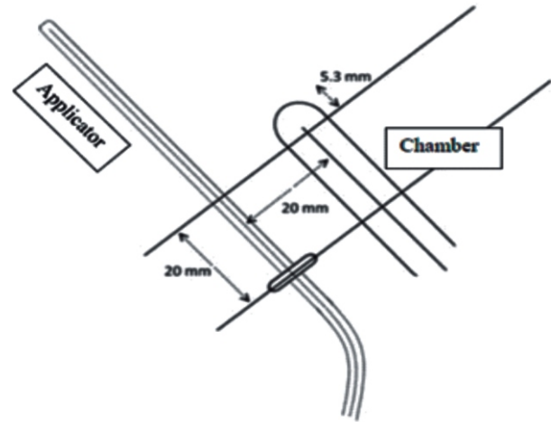
Figure 1: Experimental arrangement of the HDR applicator and chamber in the phantom.
